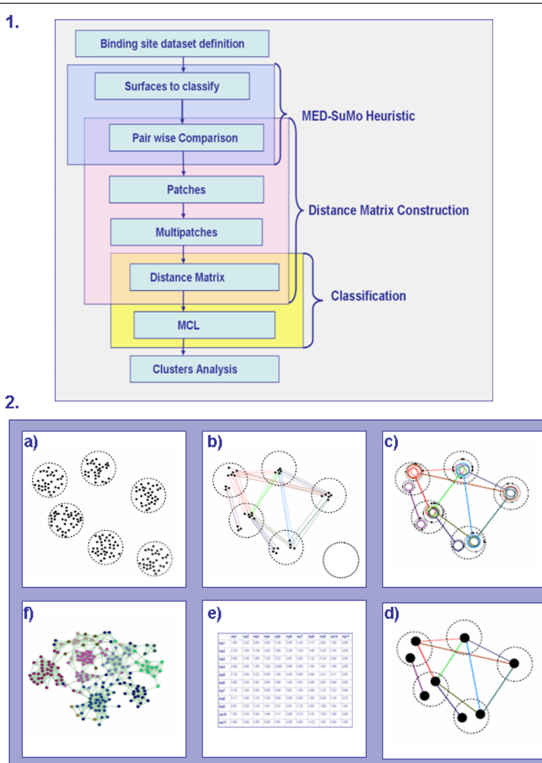
Figure 2 - MED-SuMo Classification Procedure.
