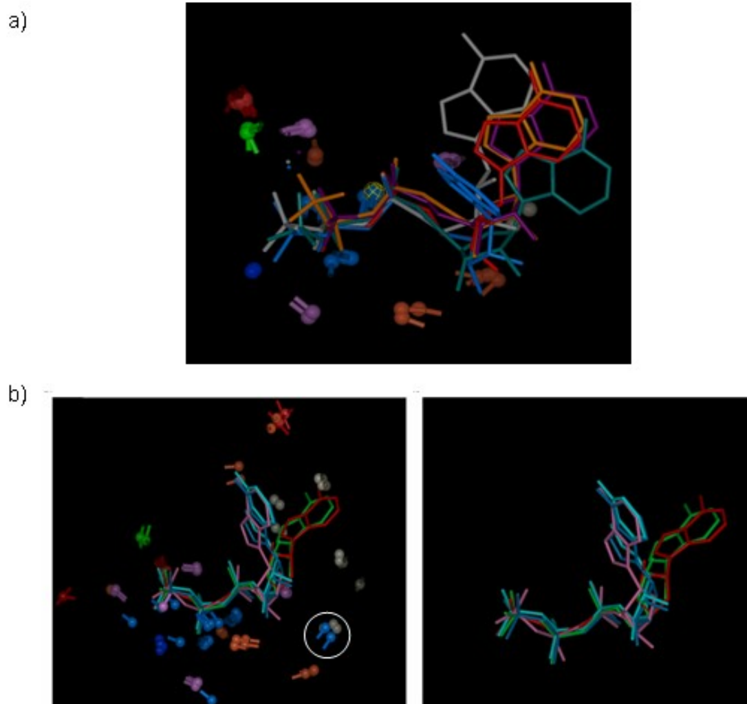
Figure 4 - Superimposition of 6 ligands from cluster 33.
