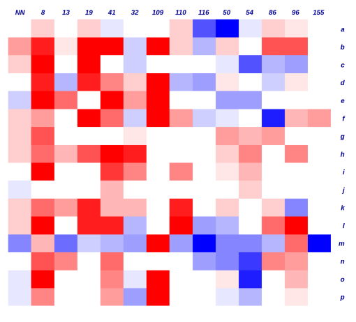
b) Interaction matrices for direct polar contacts in Umb-R1 (top), TrF-R1 (middle), and Nuc-R1 (bottom). Numbers of contacts are on the left, log-odds on the right.
