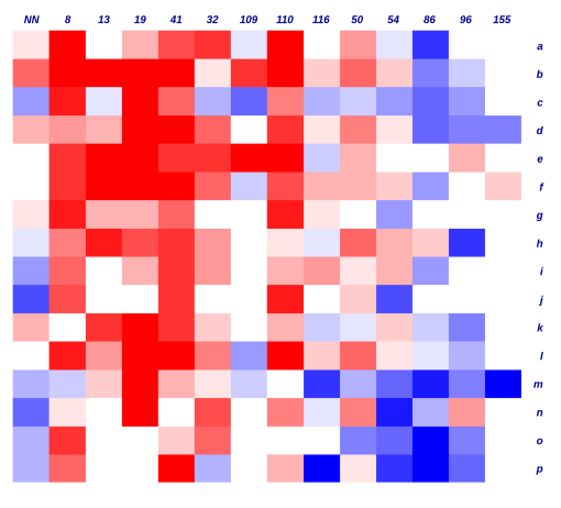
a) Interaction matrices for water-mediated contacts in Umb-R2 (top), TrF-R2 (middle), and Nuc-R2 (bottom). Numbers of contacts are on the left, log-odds on the right.
