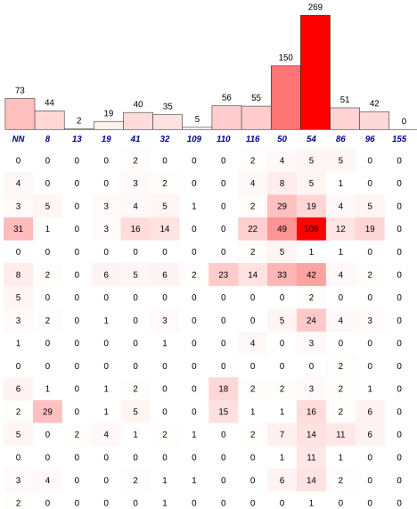
d) Interaction matrices for direct polar contacts to the major groove in Umb-R2 (top), TrF-R2 (middle), and Nuc-R2 (bottom). Numbers of contacts are on the left, log-odds on the right.
