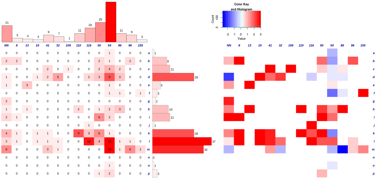
c) Interaction matrices for direct polar contacts to the minor groove in Umb-R2 (top), TrF-R2 (middle), and Nuc-R2 (bottom). Numbers of contacts are on the left, log-odds on the right.
